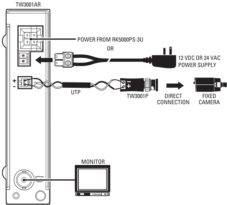
Figure 7. TW3001AR Connected to a Single Passive Transceiver
